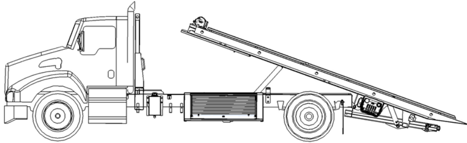
FIGURE 19 – INCLINER LE PLANCHER
