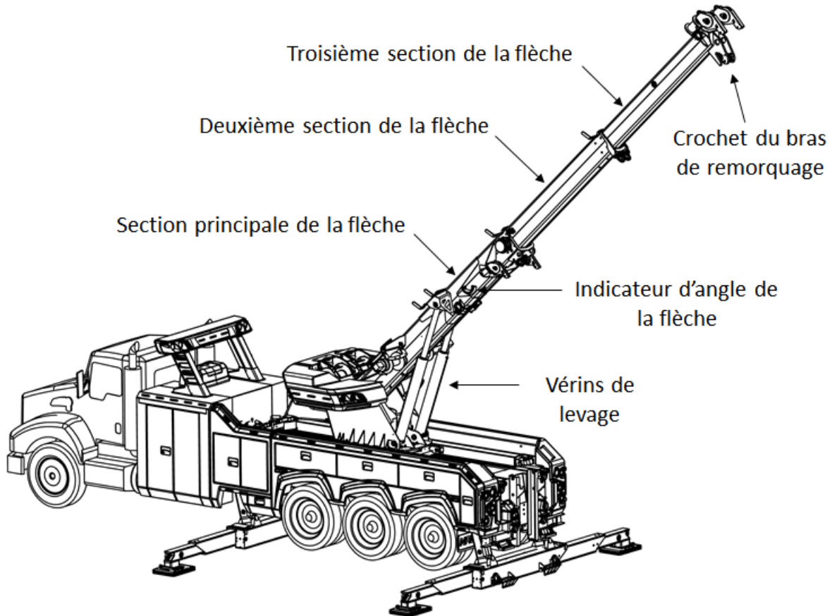
FIGURE 3 – FLÈCHE (EXEMPLE)
